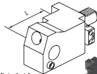
Single site, left 115-54144 (L=100) 115-54146 (L=120)
